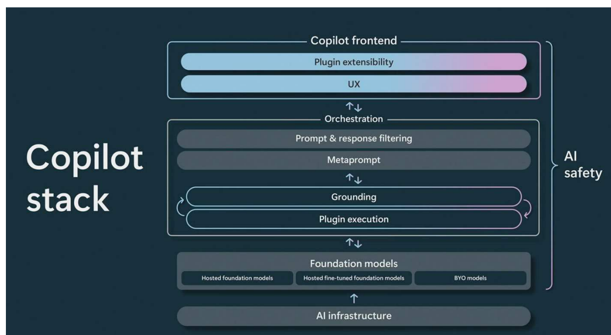
Figure 1: Copilot Stack
